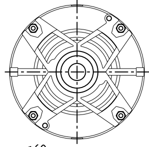
VIEW SHOWING P.F.E. VENTILATION OPENINGS
